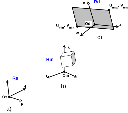
Figure 2. Scene coordinate system with a) Source R_S frame, b) Object R_m frame and c) Detector R_d frame
